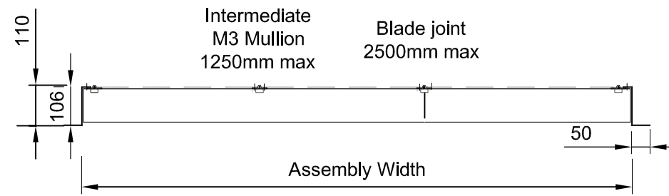
Flanged Assembly Horizontal Section
