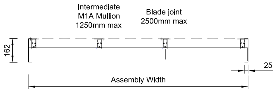
Framed Assembly Horizontal Section
