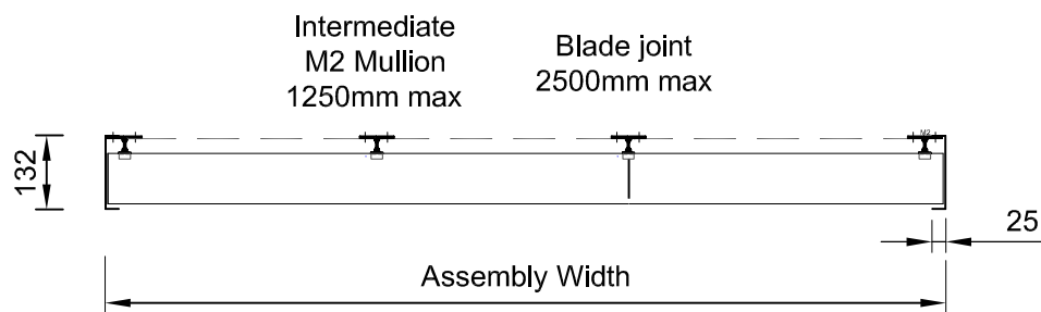
Framed Assembly Horizontal Section
