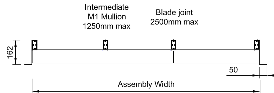
Flanged Assembly Horizontal Section
