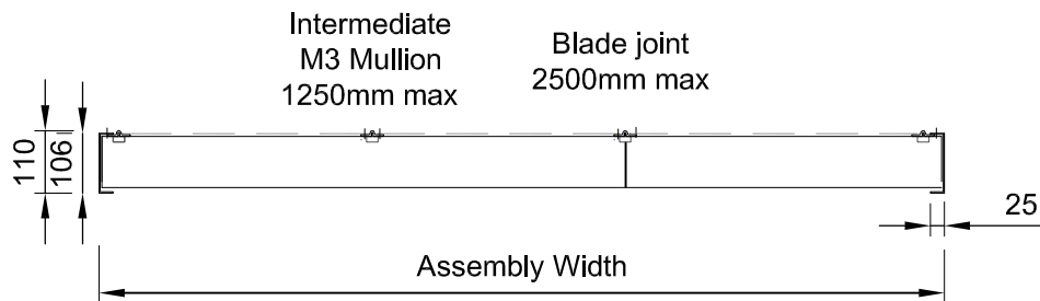
Framed Assembly Horizontal Section
