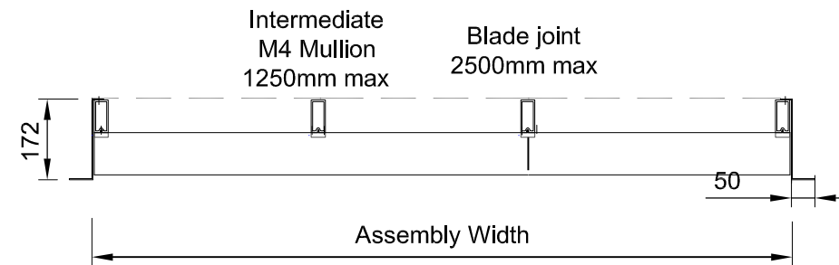
Flanged Assembly Horizontal Section
