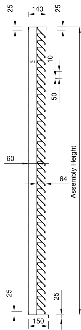
Framed Assembly Vertical Section
