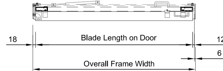
Single Door Horizontal Section
