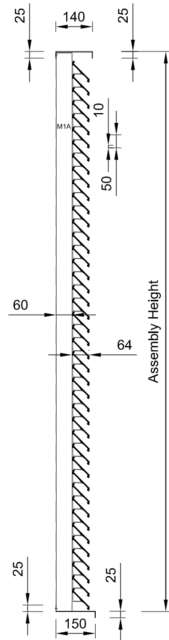
Framed Assembly Vertical Section
