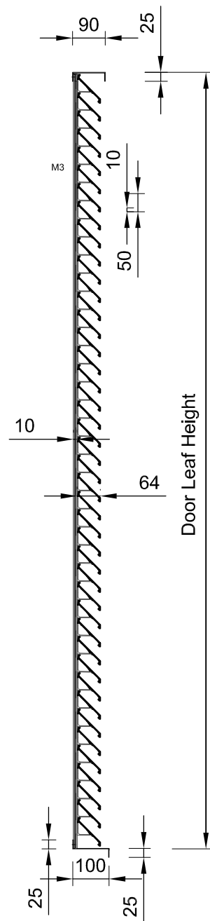
Framed Assembly Vertical Section
