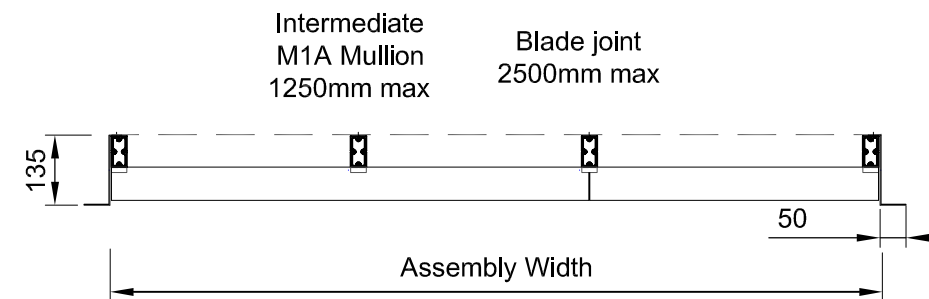
Flanged Assembly Horizontal Section
