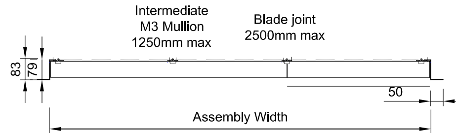
Flanged Assembly Horizontal Section
