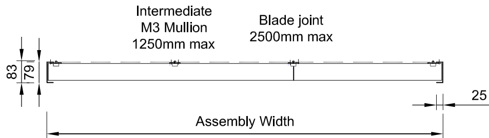
Framed Assembly Horizontal Section
