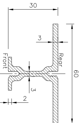
M2 Mullion
