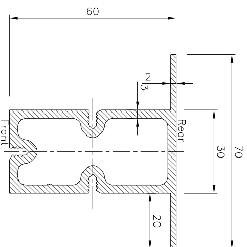
M1A Mullion
